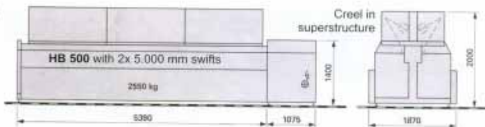
Dimensional drawing (measurements in mm)
